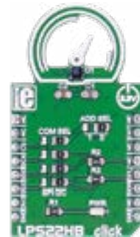
LPS22HB Click Used as a digital barometer. It carries the LPS22HB MEMS nano pressure sensor.
