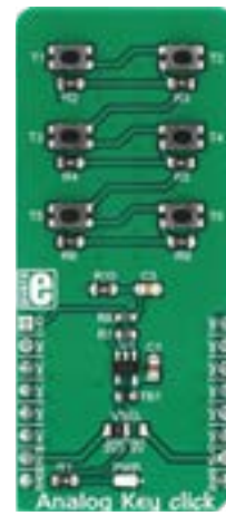
Analog Key Click The KMR2 series KMR221 tactile buttons are high-quality SPST switches produced by CKSwitches. MSRP - $14 00 MIKROE-3409
