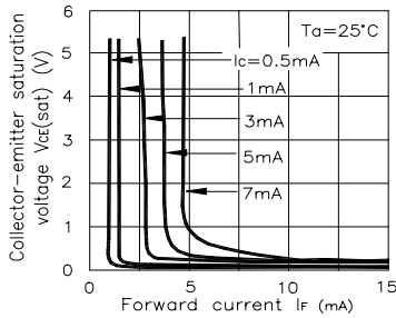
Fig. 11 Collector-emitter Saturation Voltage vs. Forward Current
