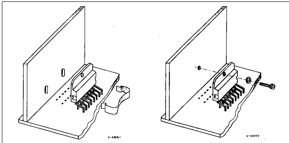
Figure 5 : Mounting Examples
