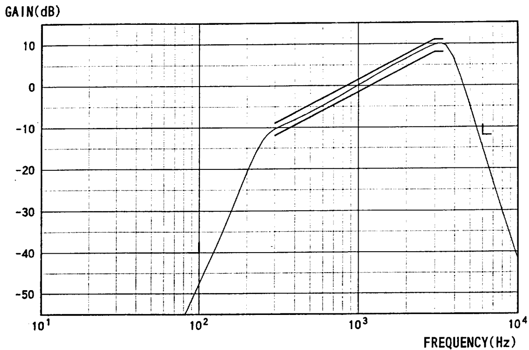
Fig. 1 Transmission overall characteristics
