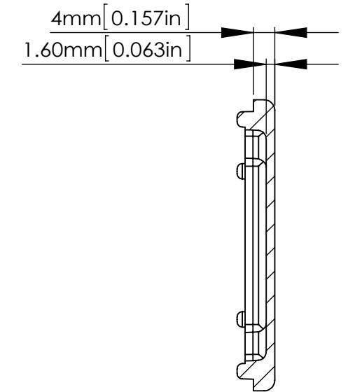
SECTION B-B SCALE 1 : 1
