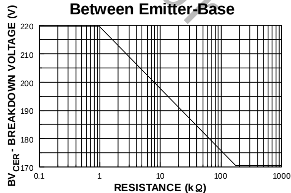
Collector-Emitter Breakdown Voltage with Resistance Between Emitter-Base
