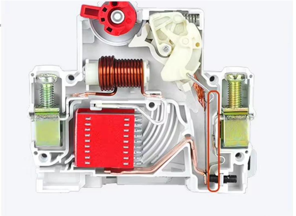
Arc-extinguishing room, swift arc breaking
