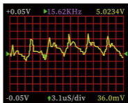
High-speed voltage ripple (AC coupling)
