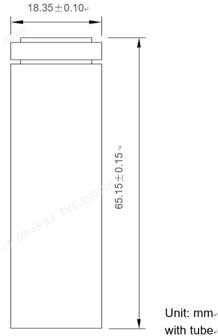
Fig. 1. Outline Dimensions of INR18650/30P
