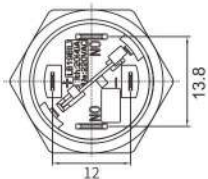
Outline Dimension
