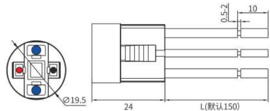
● LED 0.5mm 2 ● NO 1mm 2 Connector: Cable length: 150mm, Other lengths can be customized Connector
