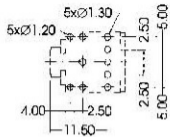
PIERCING PLAN
