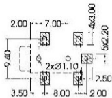
PIERCING PLAN
