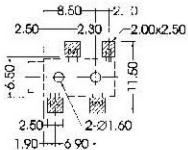
PIERCING PLAN
