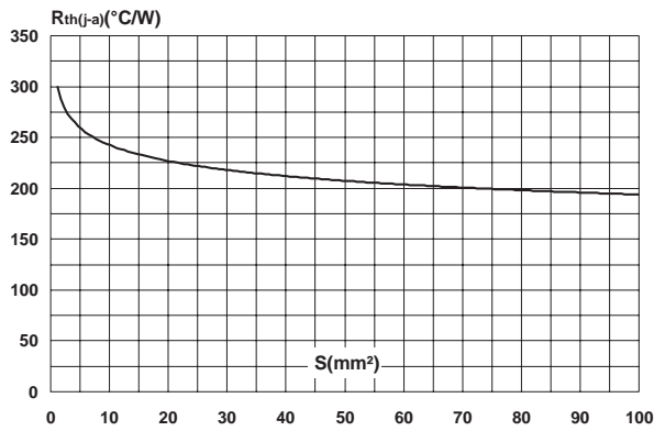
Fig. 9: Thermal resistance junction to ambient versus copper surface under each lead (epoxy printed board FR4, \text{Cu}=35\mu\text{m} , typical values).
