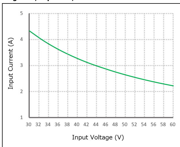
Figure 3, Input V-I, Iout=10A
