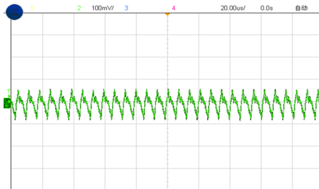
Figure 7, Output ripple & noise ( I_{out} = 10\text{A} )
