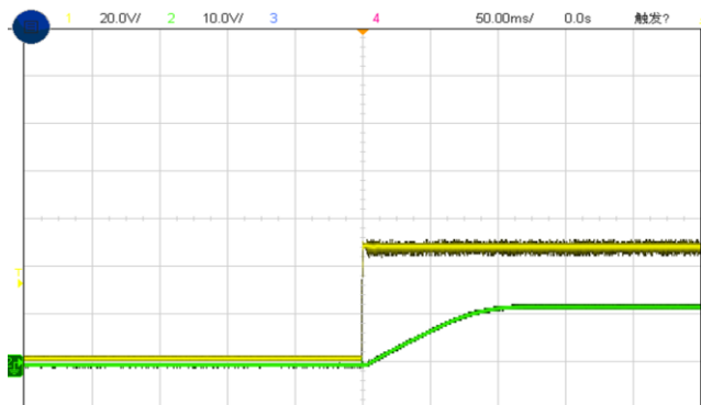
Figure 6, Output voltage established ( I_{out} = 10\text{A} )
