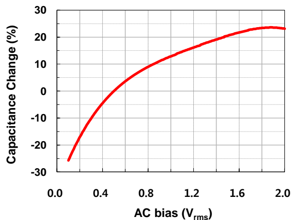
- Capacitance Change(%) with AC bias
