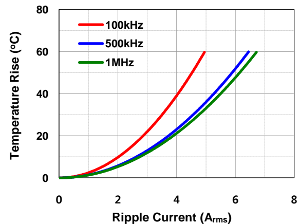
- Temperature Rise with Ripple Current
