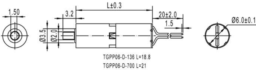
Gear Motor Dimensions (mm)
