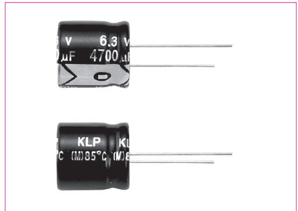
Marking color: white print on black sleeve
