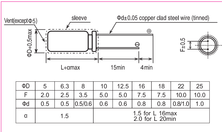
Outline Drawing
