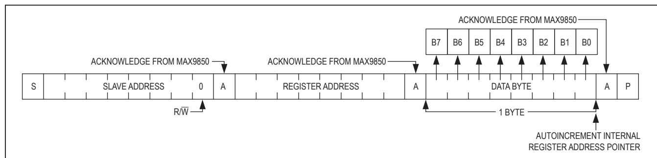
Figure 8. Writing One Byte of Data to the MAX9850
