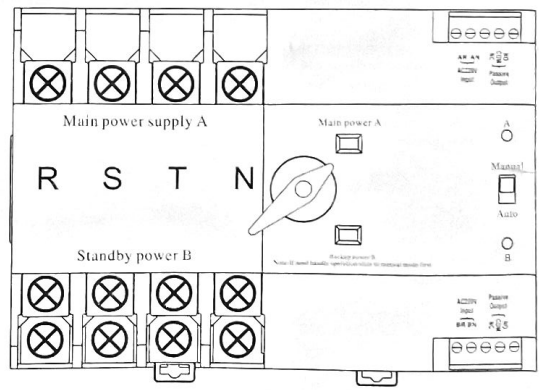
Picture 4 Correct mounting direction
