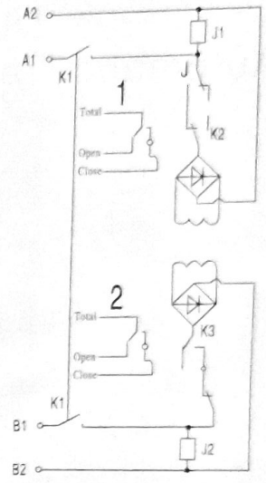
Picture 2 Internal wiring diagram
