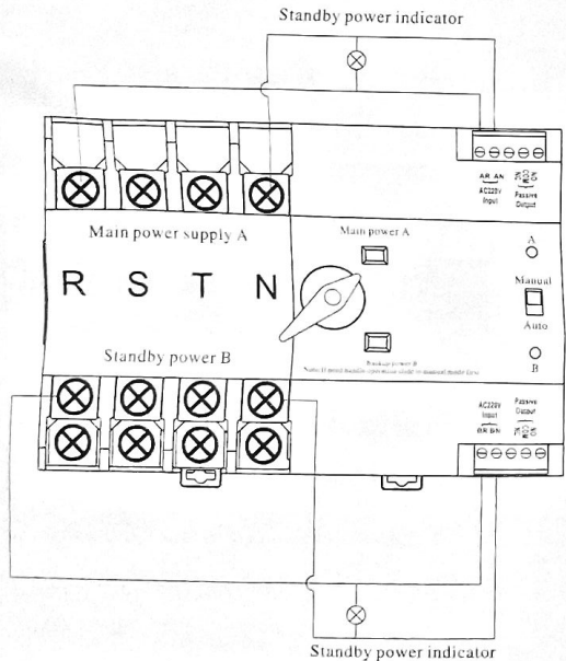
Picture 3 Controller wiring diagram
