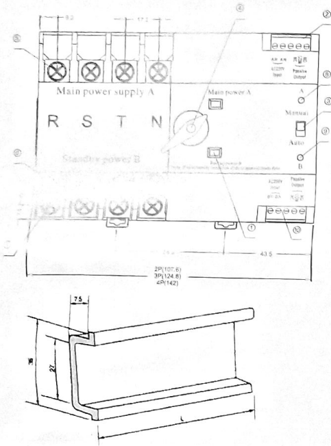
Picture 1 Appearance dimensions and Installation dimensions
