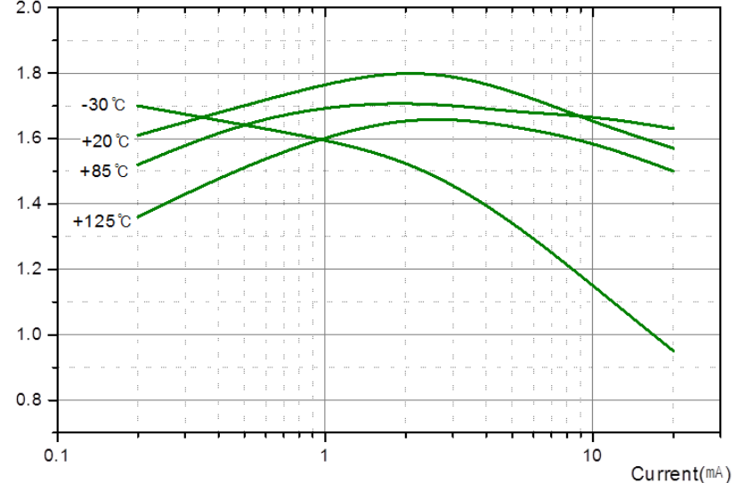
Capacity(Ah) Capacity versus Current
